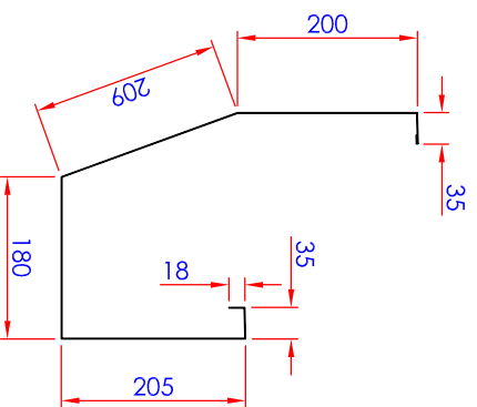
Double Sided Plastisol Gutter (B) (1:10)
