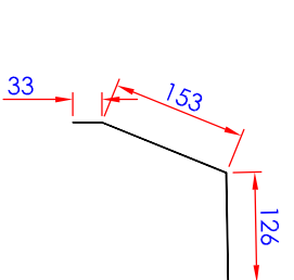
0.7mm Galvanised Steel Flashing (A) (1:10)
