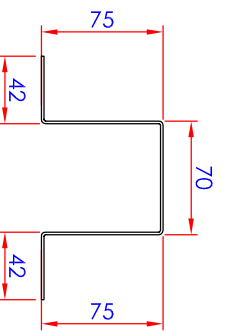
Galvanised Steel Top Hat (C) (1:5)
