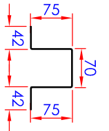
1.6mm Galv Steel Top Hat 75mm Deep (A)
