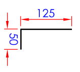
1.6mm Galv Steel Closure Angle (F)
