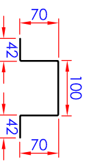
1.6mm Galv Steel Top Hat 75mm Deep (C)
