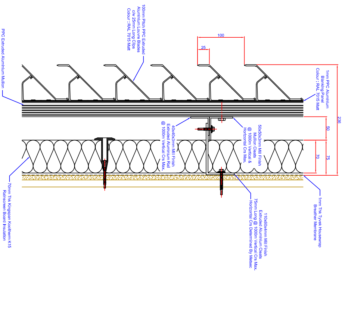
TYPICAL SECTION THROUGH NON-ACTIVE STANDARD LOUVRE 1:2.5
