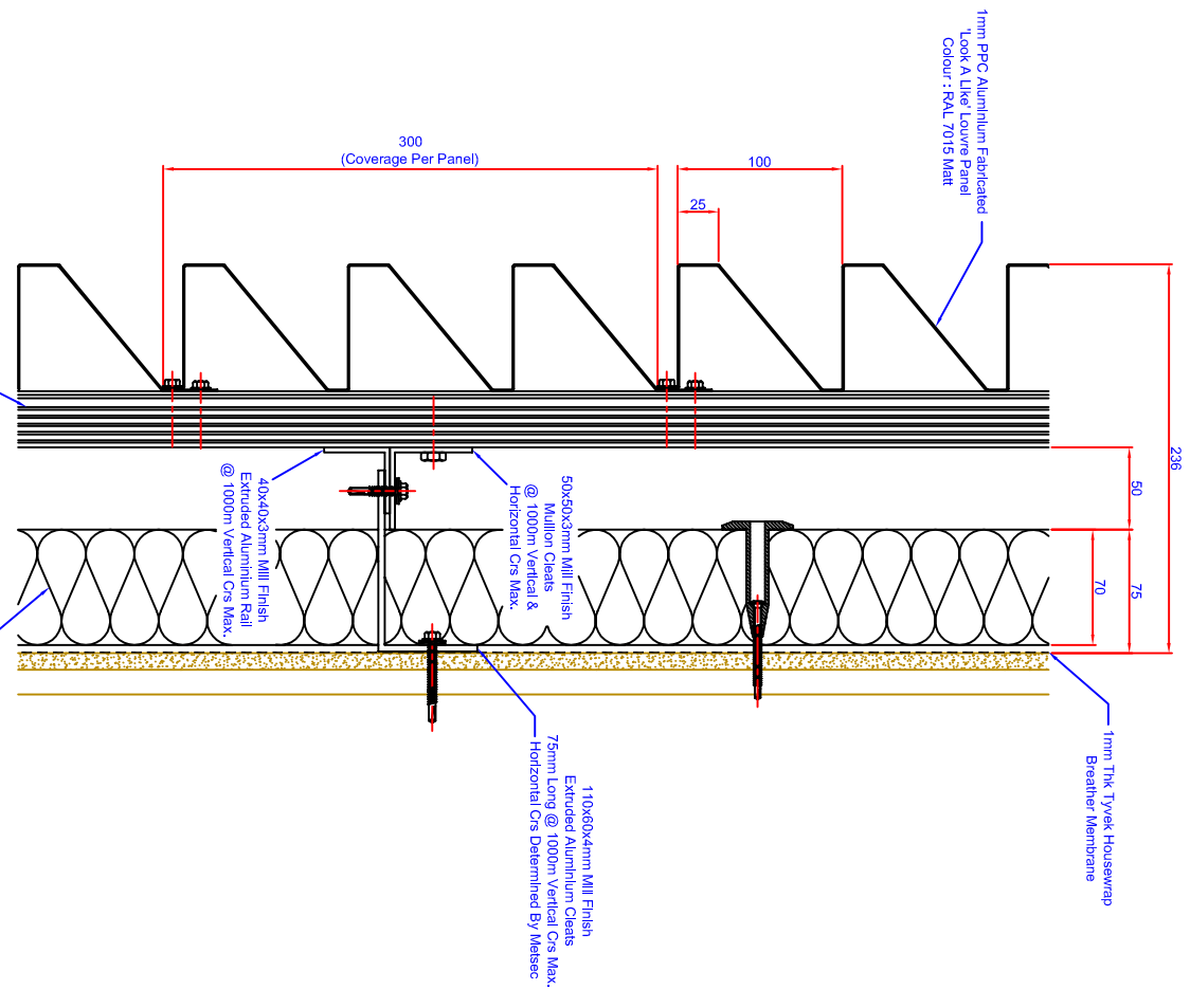
TYPICAL SECTION THROUGH ACTIVE CHEVRON LOUVRE 1:2.5
